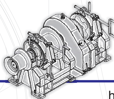
hydraulic ramp winch
